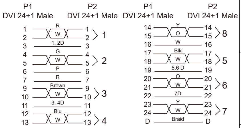
Pin Assignment
