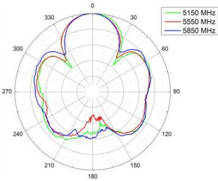
Port1: E-Plane
