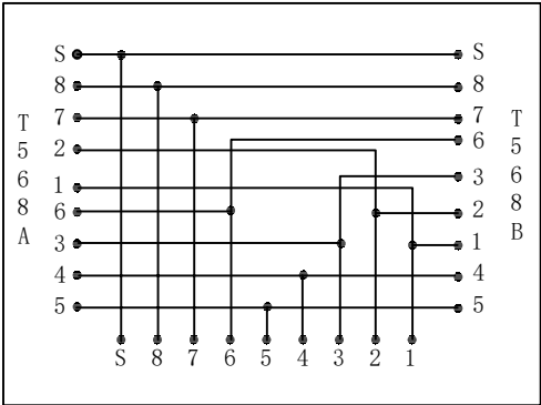
Pin Out:
