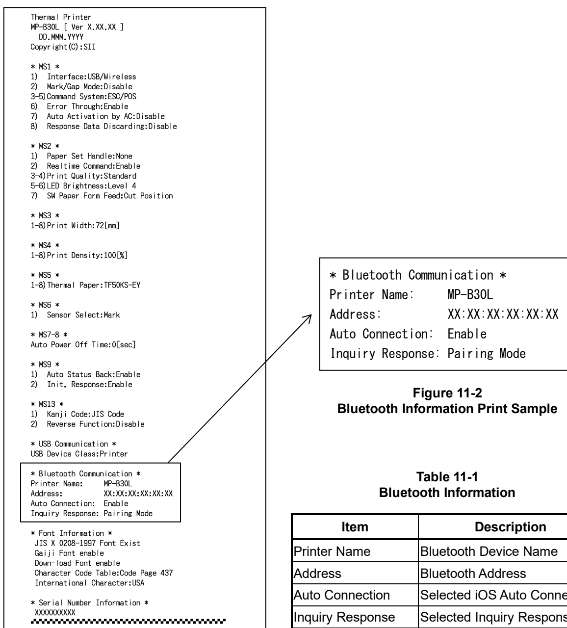
Figure 11-1 Test Print Sample (Bluetooth Model)
