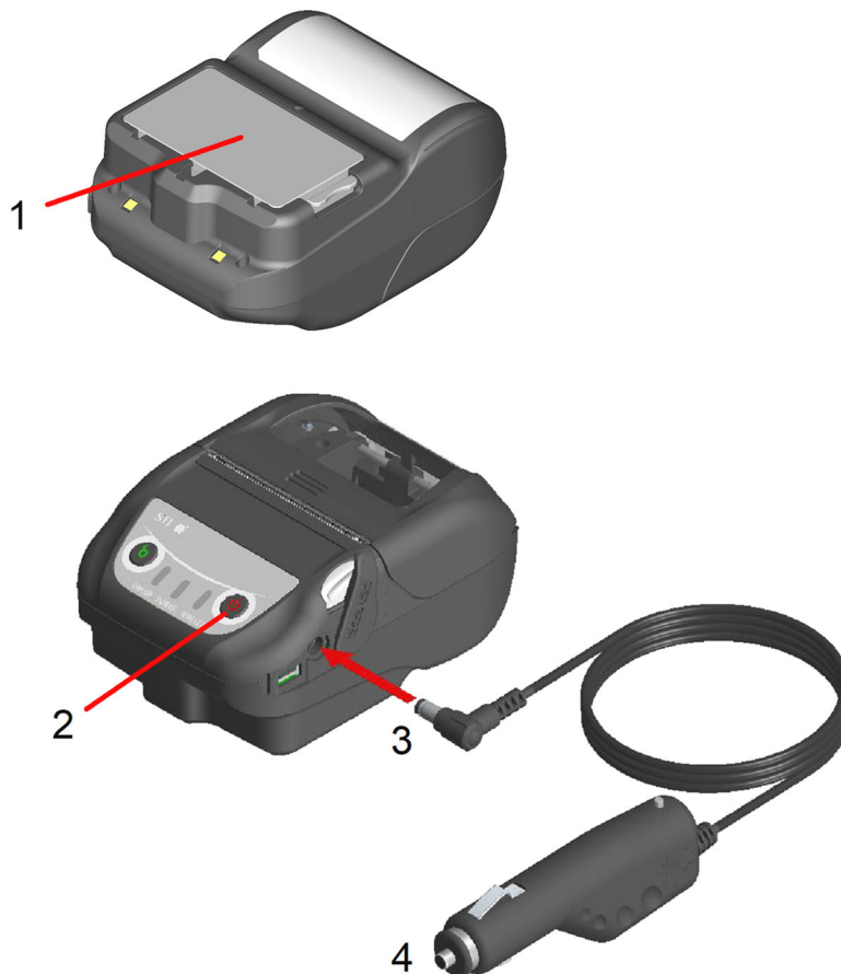
Figure 18-2 Charging in Power On Charging Mode from Car Charger
