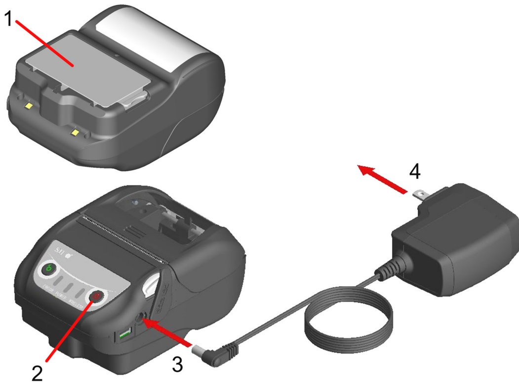
Figure 16-1 Charging in Power On Charging Mode from AC Adapter
