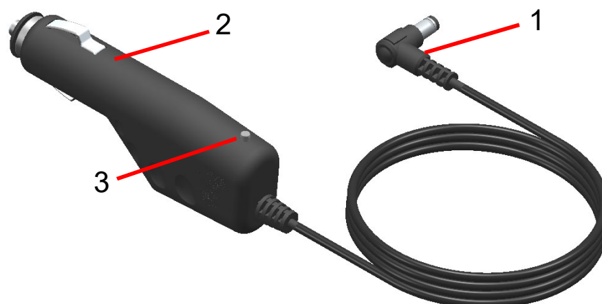
Figure 18-1 Each Part of Car Charger (CC-A12-A1)
