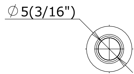
Detail Z (2 : 1) Hole size (Position B,D,E,F)
