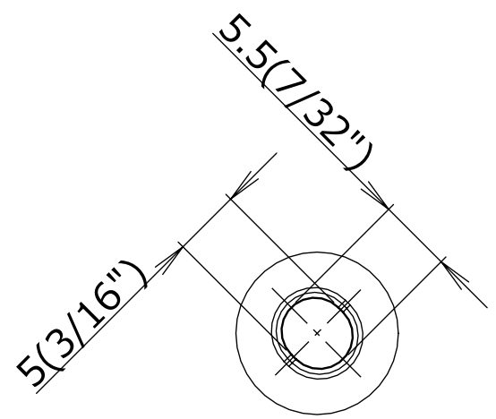
Detail Y (2 : 1) Hole size (Position A,C)
