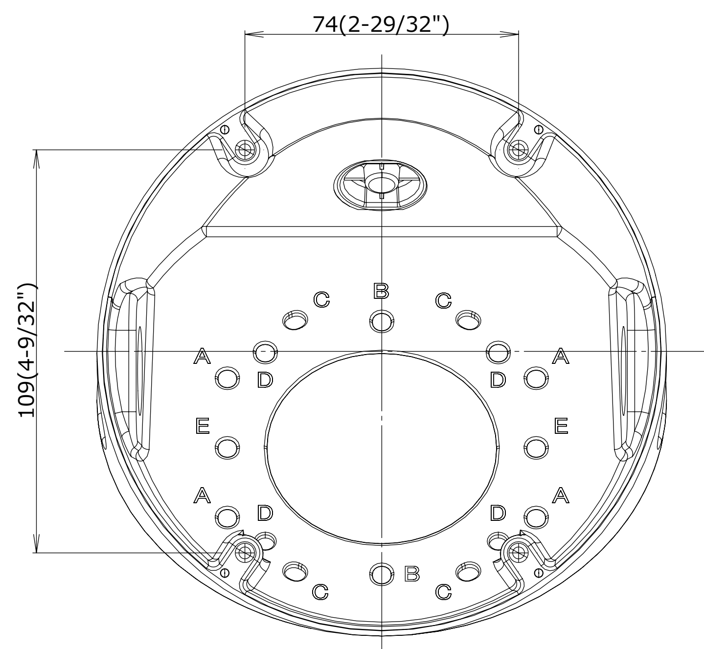
View B
